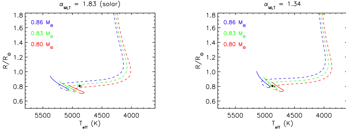
Figure 4. Radius-temperature plot showing the position of HD 189733 with 1\text{-}\sigma errors (black point). Each panel also shows evolutionary tracks for the mass indicated in legend, corresponding to the mass of HD 189733 (green), and a range above (blue) and below (red) this value by \sim 1\text{-}\sigma of the MC analysis. Dashed and solid lines denote pre-main sequence and main sequence evolutionary stages, respectively. The left panel are models using the solar calibrated \alpha_{\text{MLT}} , and the right panel is \alpha_{\text{MLT}} parameter found in this work. Note, only models with a reduced \alpha_{\text{MLT}} reproduce the observed stellar properties for HD 189733 as a main-sequence star. For details, see Section 5.3.1 and 5.3.2.
