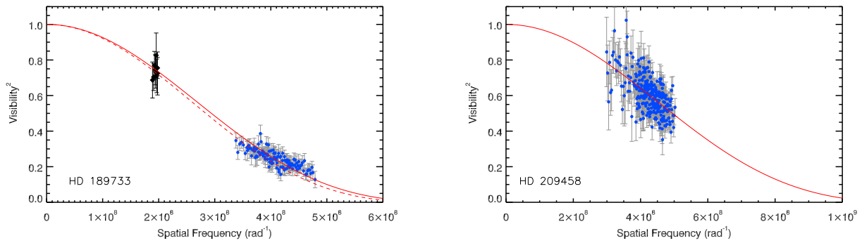
Figure 1. Plots of calibrated interferometric V^2 values and the limb-darkened V^2 values for HD 189733 (left) and HD 209458 (right). The blue dots are data presented in this work and the solid red line is the R -band limb-darkened diameter fit for each star. The black diamonds are the data from Baines et al. (2007), and the dashed red line represents their H -band limb-darkened diameter fit. Note that the V^2 functions are different for HD 189733 due to the limb-darkening coefficient, which is larger in R -band compared to H -band. The interferometric observations are described in Section 2.1.
