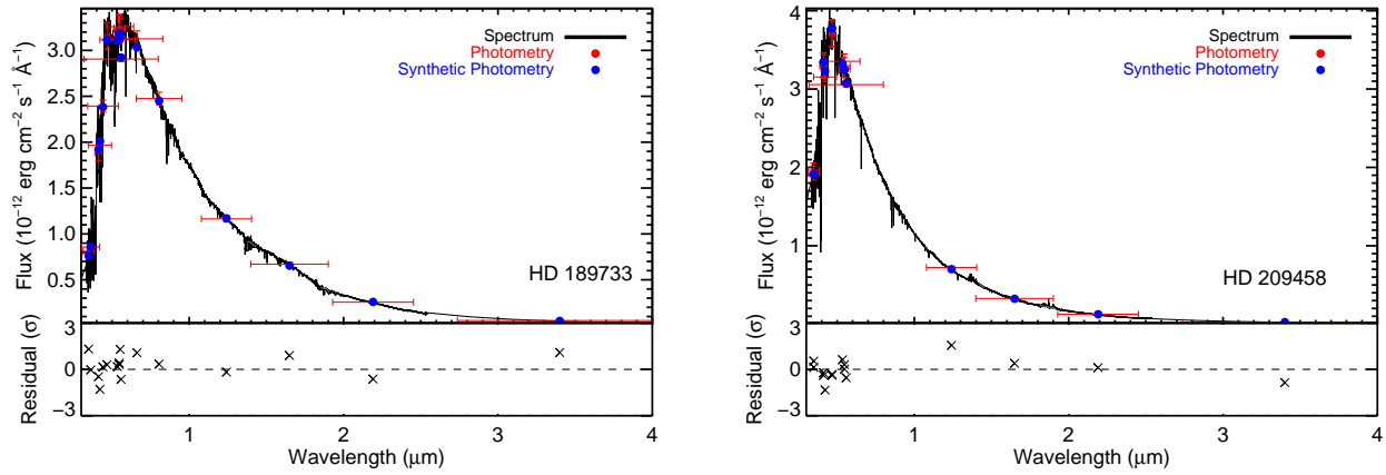
Figure 2. SED’s for HD 189733 (left) and HD 209458 (right). The (black) spectra represent the joined SNIFS+uSpeX spectra. The (red) points indicate photometry values from the literature. “Error bars” in x-direction represent bandwidths of the filters used. The (blue) points show the flux value of the spectral template integrated over the filter transmission. The lower panel shows the residuals around the fit in units of standard deviations. For details, see Section 2.3, and for results, see Table 3.
