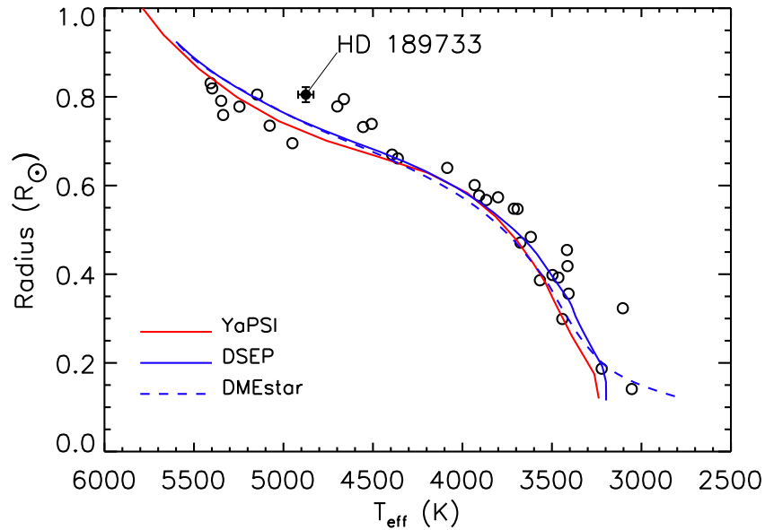
Figure 3. Radius - temperature plot showing the position of HD 189733 (filled point) with the low-mass stars in Boyajian et al. (2012) (open points). Also plotted are solar abundance, 5 Gyr isochrones from the DSEP (solid blue line), DMEstar (dashed blue line), and YaPSI (solid red line) model grids. Refer to Section 4 for details.
