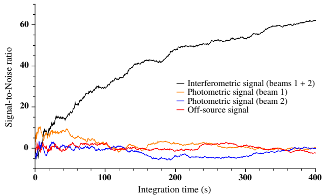
FIG. 3. Comparison of the signal-to-noise ratio measured in interferometric and in photometric configurations. In the photometric configurations, the flux level is measured by injecting the light in one single arm, one after the other, and then without light injection at the input of the interferometer.
