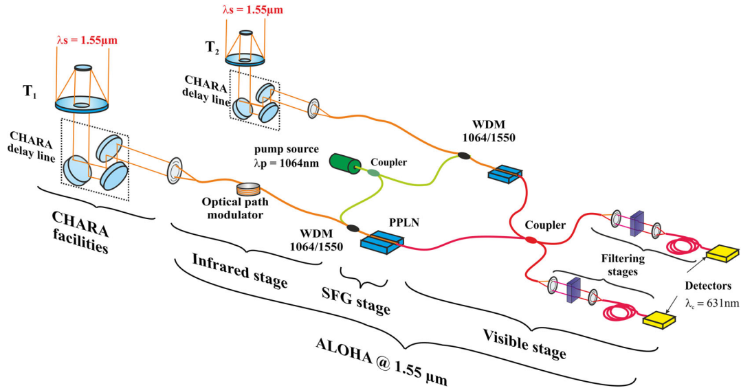
FIG. 1. On-site configuration with implementation of the ALOHA prototype at 1.55 \mu\text{m} on the CHARA Array. It is composed of three different stages (infrared, SFG, and visible stages). Apart from the filtering stage, the interferometer is entirely fibered with single-mode and polarization maintaining fibers.
