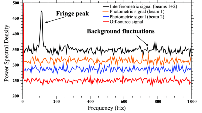
FIG. 2. Experimental power spectral density related to the \alpha UMa interferogram. Black: interferometric configuration, blue and orange: photometric signals, red: interferometric configuration without signal source.
