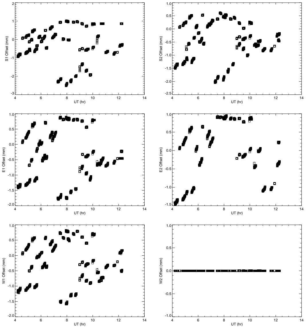
Fig. 2.— Baseline offsets vs. time for each cart on UT 2021 Jul 29, Aug 02, and Aug 06 using the new baseline solution. A few different POP configurations were used.
