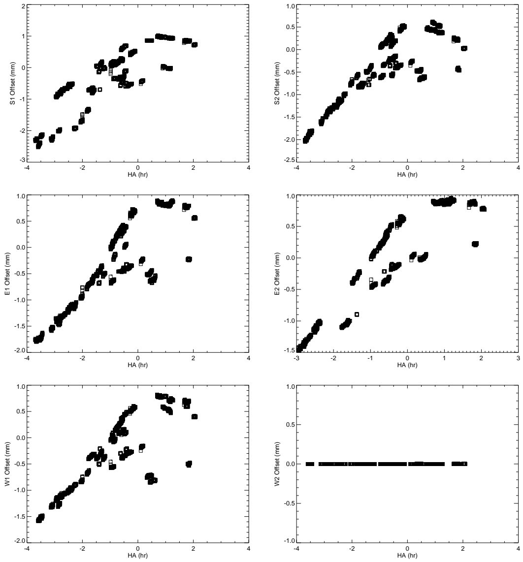
Fig. 1.— Baseline offsets vs. hour angle for each cart on UT 2021 Jul 29, Aug 02, and Aug 06 using the new baseline solution. A few different POP configurations were used.
