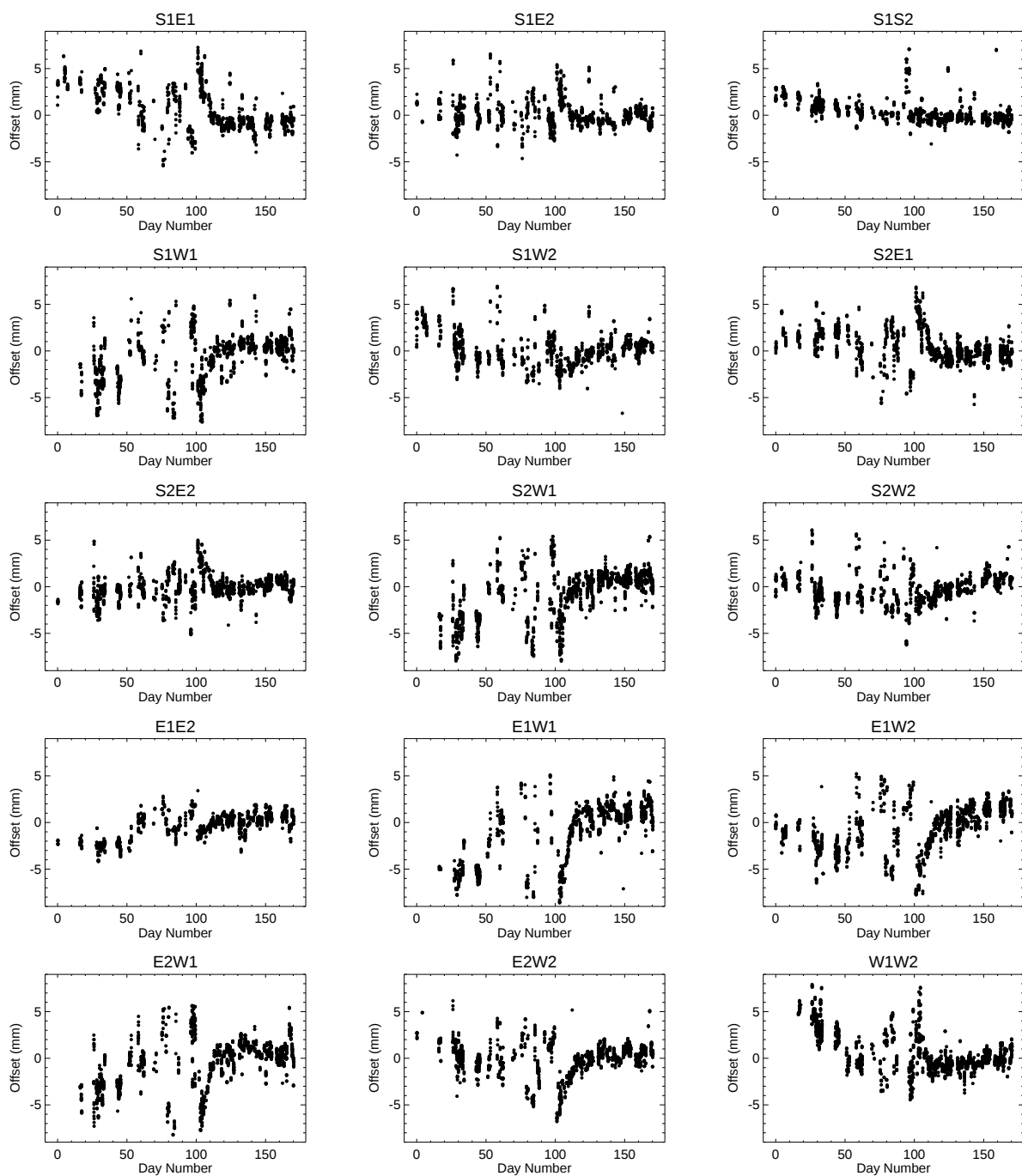
Figure 2: Residual vs. day number.
