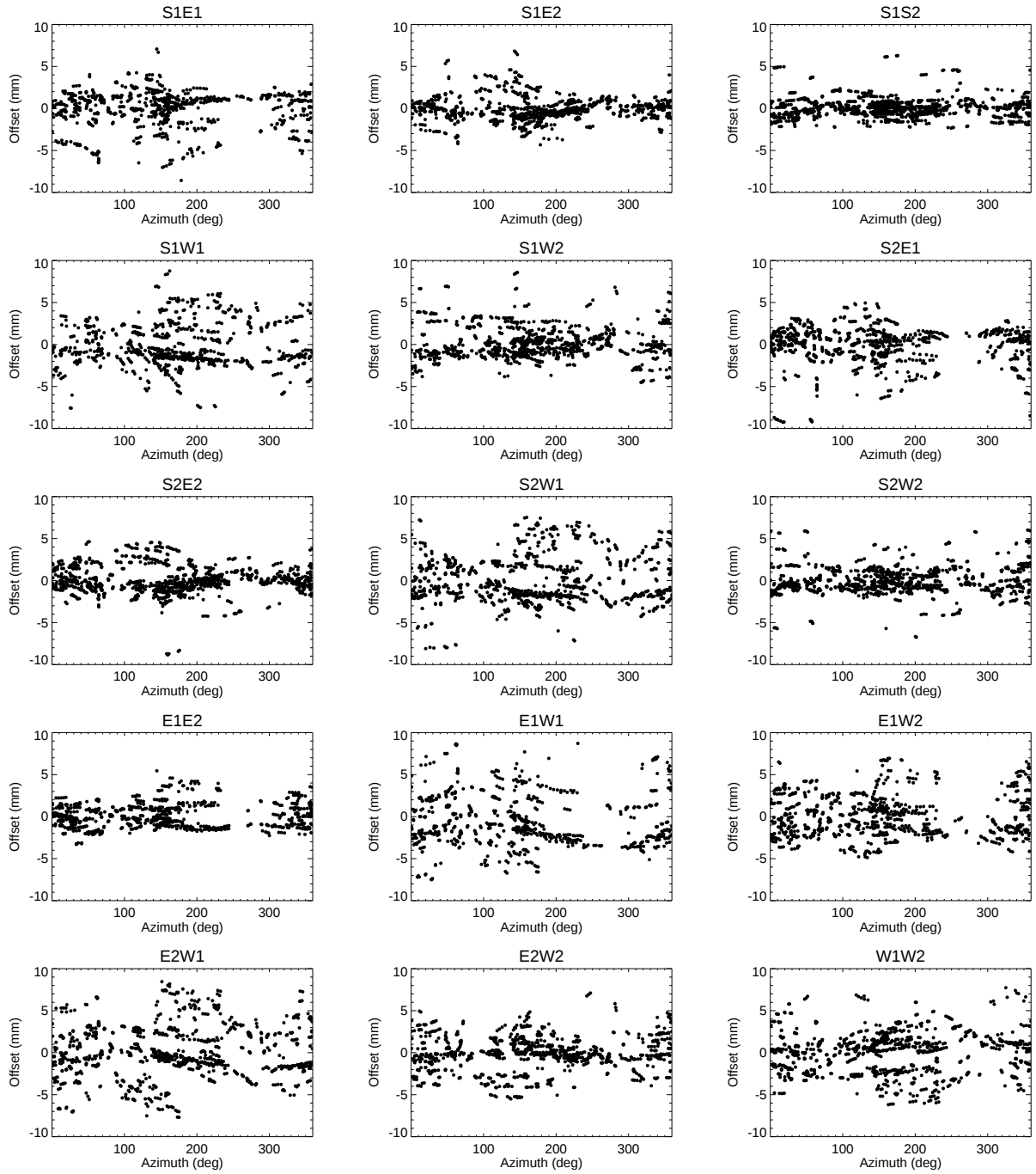
Figure 4: Residual vs. azimuth.
