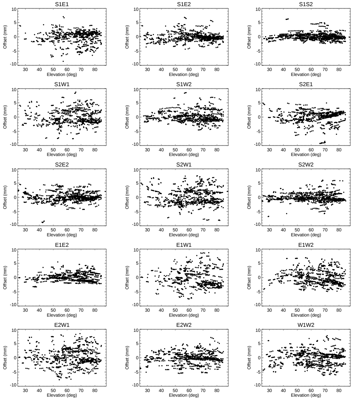
Figure 3: Residual vs. elevation.
