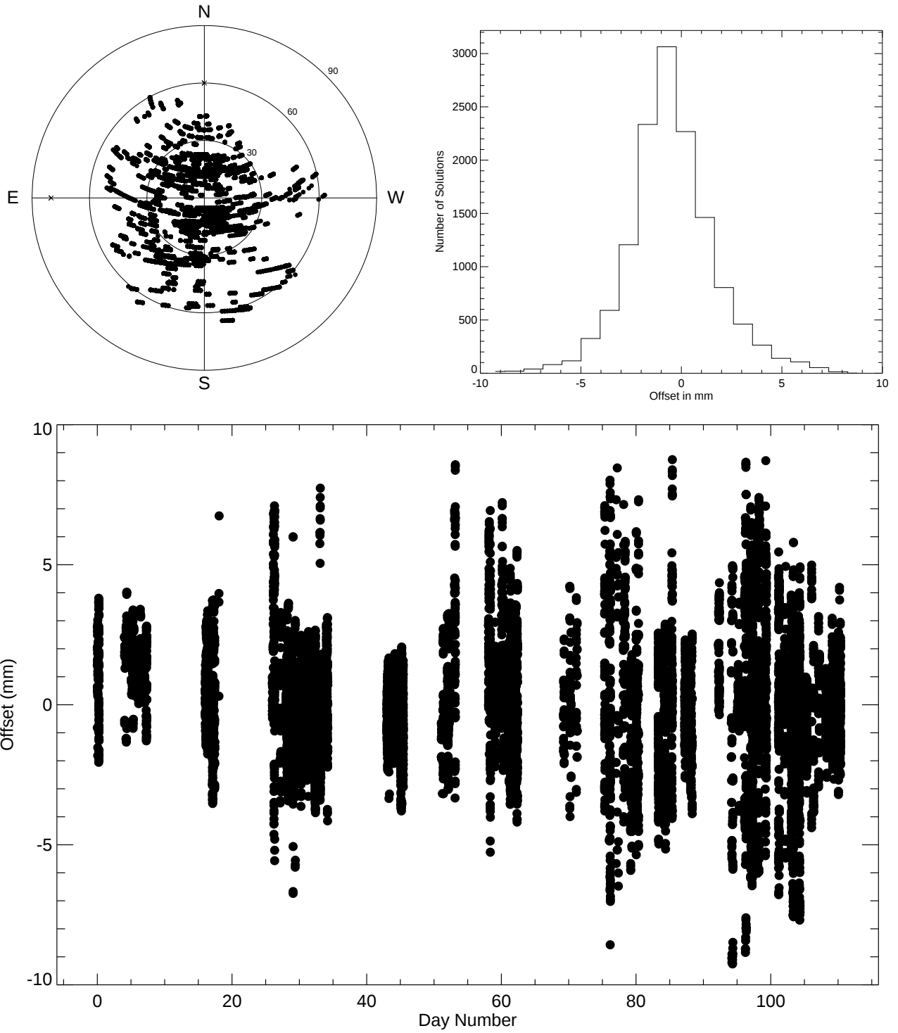
Figure 1: Top left: Sky coverage. Top right: Histogram of residuals. Bottom: Residuals vs. day number.
