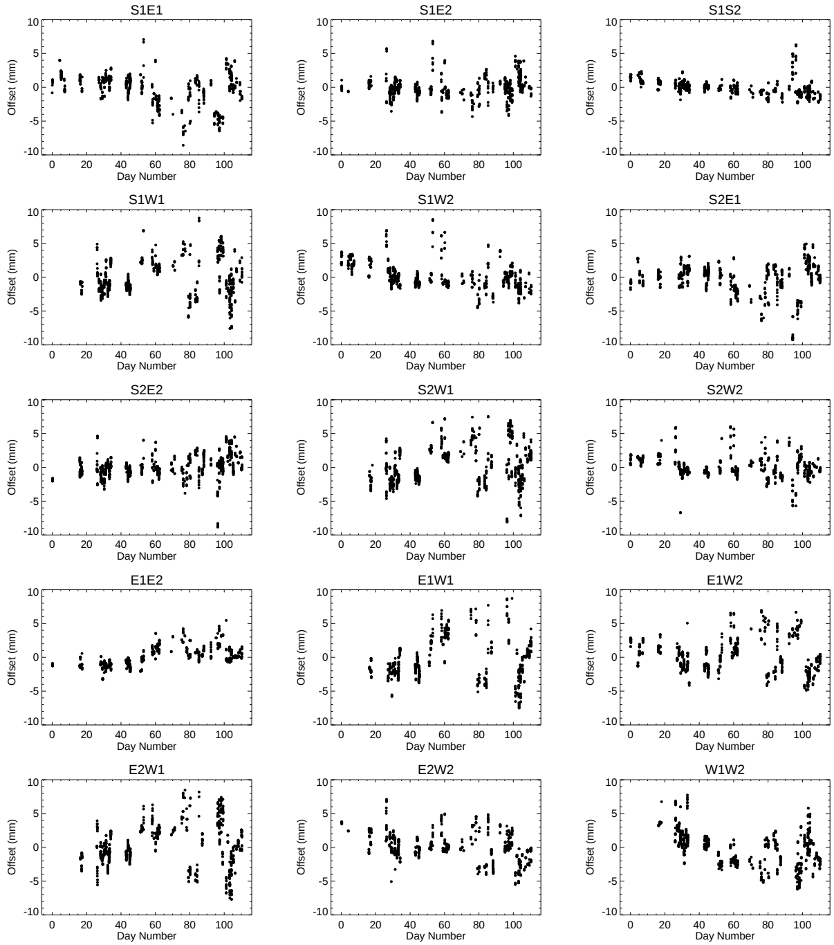
Figure 2: Residual vs. day number.
