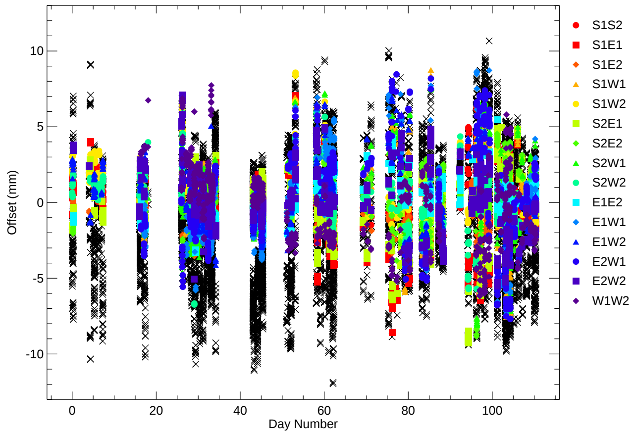
Figure 6: Residuals from the fit to the baseline solution color coded by the baseline. The black crosses indicates the offset measured on sky using the baseline solution in use at the time.
