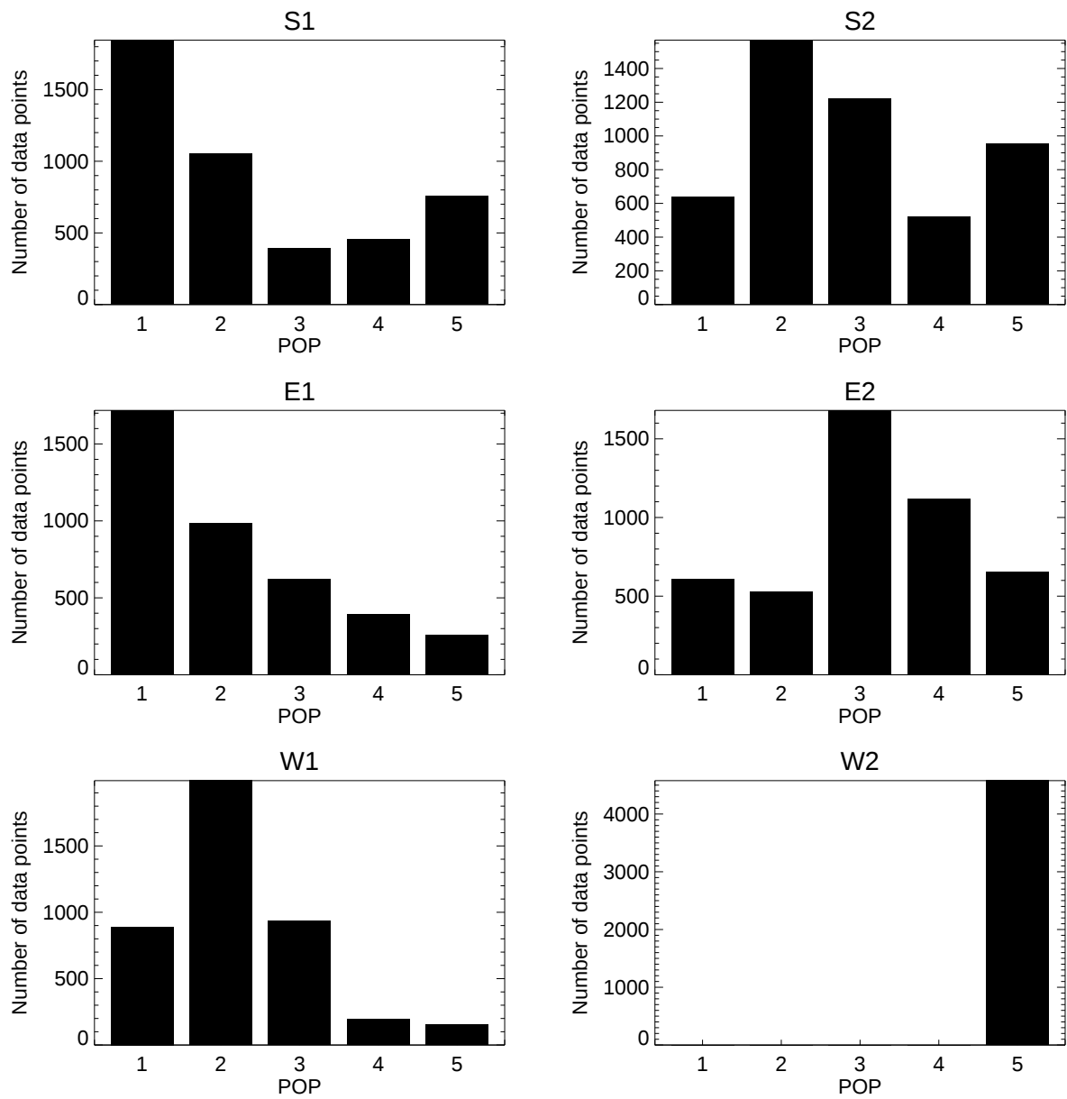
Figure 5: Number of observations on each pop
