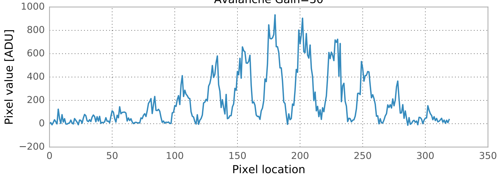
Avalanche Gain=30
