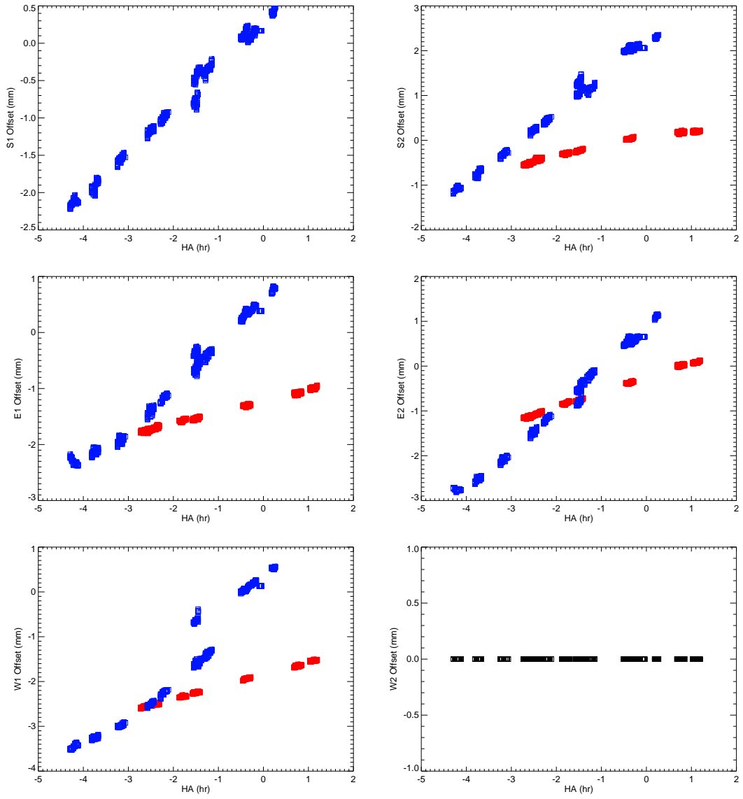
Fig. 1.— Baseline offsets vs. hour angle for each cart on UT 2021Sep17 (red) and UT 2021Sep20 (blue). Different POP configurations were used each night.
