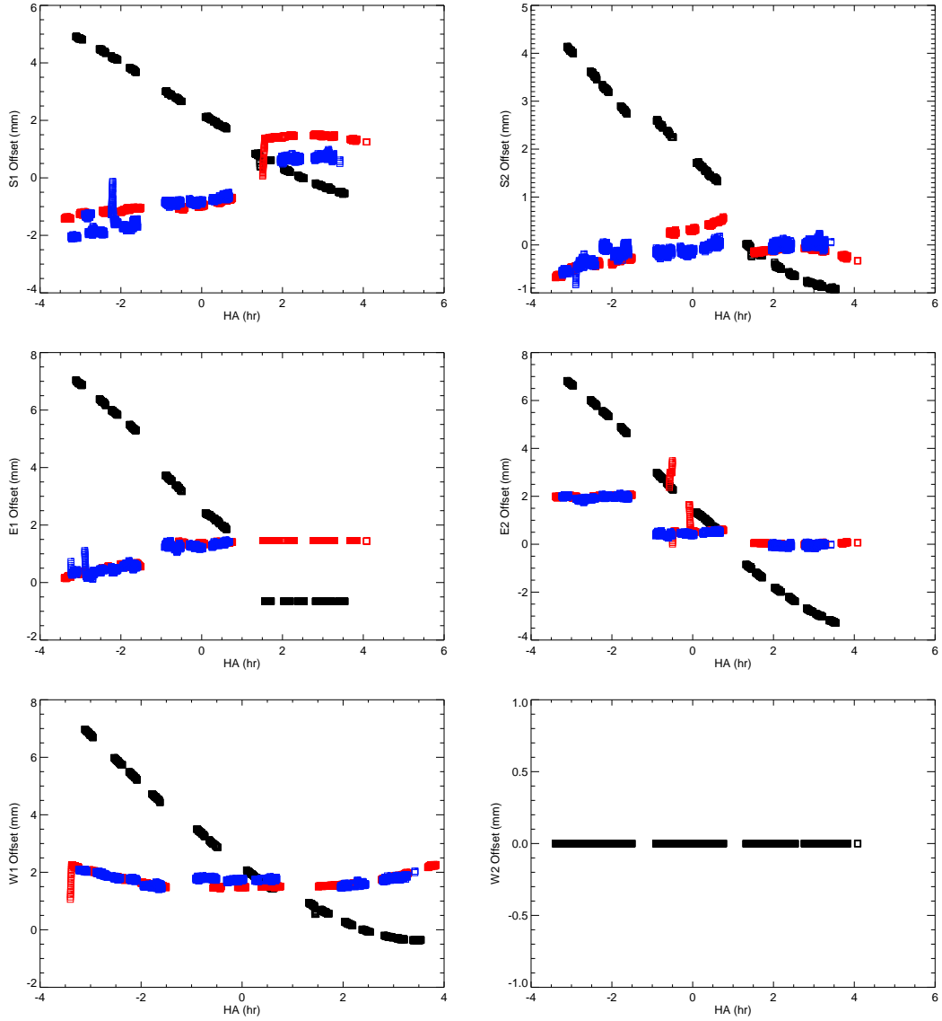
Fig. 1.— Baseline offsets vs. hour angle for each cart on using the old baseline solution on UT 2022Apr02 (black) and the new baseline solution on UT 2022Apr03 (red) and UT 2022Apr04 (blue).
