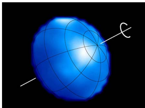
Figure 1: Image of the surface of Altair from CHARA observations (from Monnier et al, Science, 2007, 317, 342).
