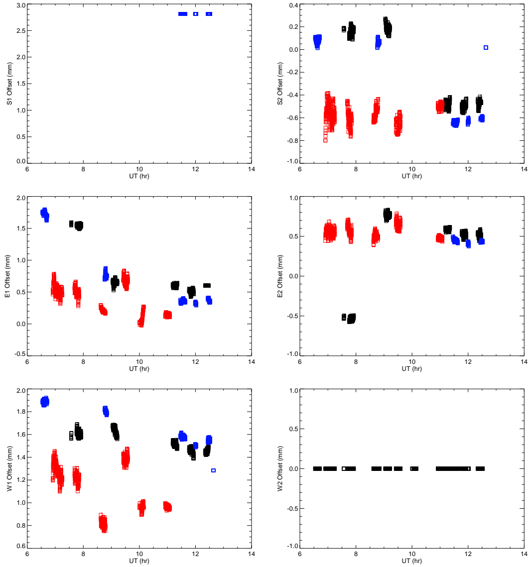
Fig. 3.— Baseline offsets vs. time for each cart on UT 2022 May 22 (black), 23 (red), and 24 (blue).
