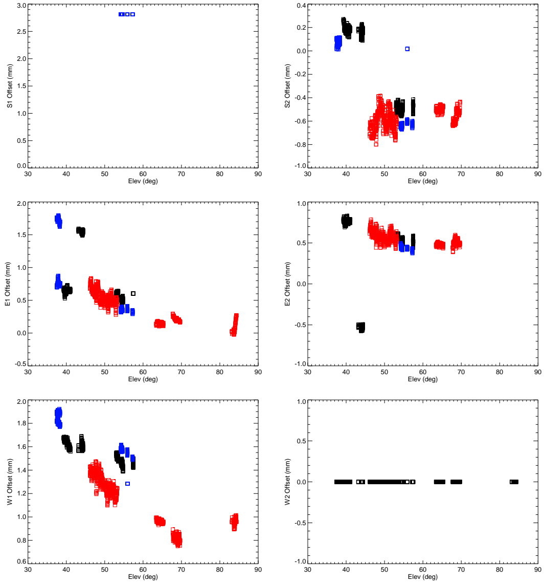
Fig. 2.— Baseline offsets vs. elevation for each cart on UT 2022 May 22 (black), 23 (red), and 24 (blue).
