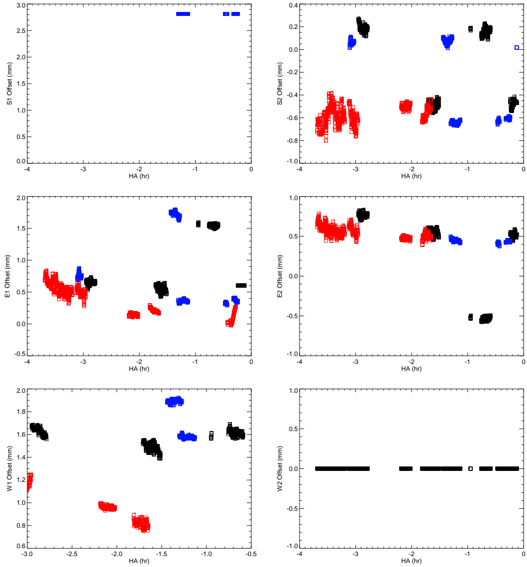
Fig. 1.— Baseline offsets vs. hour angle for each cart on UT 2022 May 22 (black), 23 (red), and 24 (blue).
