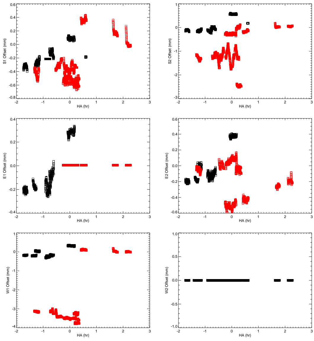
Fig. 1.— Baseline offsets vs. hour angle for each cart on UT 2022 Jun 19 (black) and 20 (red).
