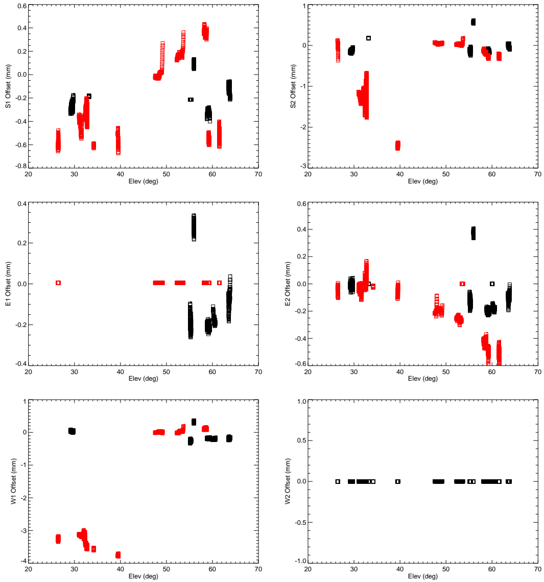
Fig. 2.— Baseline offsets vs. elevation for each cart on UT 2022 Jun 19 (black) and 20 (red).
