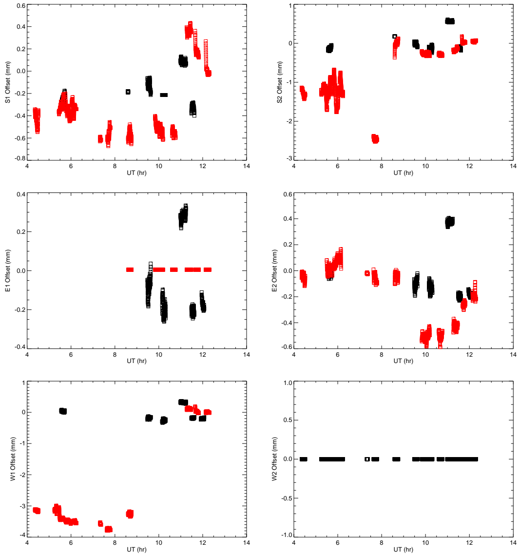
Fig. 3.— Baseline offsets vs. time for each cart on UT 2022 Jun 19 (black) and 20 (red).
